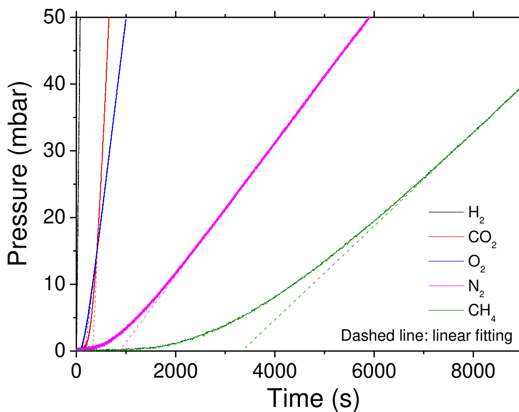
Fig. S2 A representative pressure-time profile of gas permeation for a Matrimid®/ZIF-8-30wt% sample (annealed at 230°C for 18h under vacuum). The dashed lines represent the linear fitting of the steady state. Gas permeation test condition: feeding pressure of 4 bar at room temperature (22°C).
