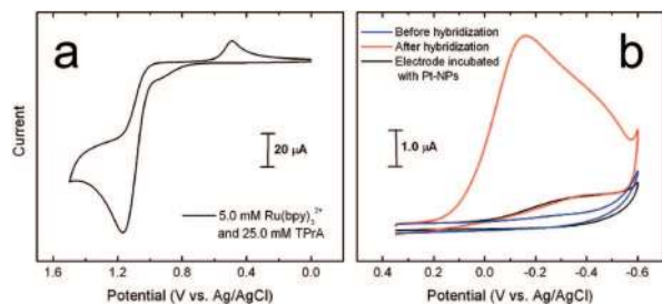
Figure 2. Cyclic voltammograms obtained from a macroscopic gold working electrode configured within a standard three-electrode cell. (a) The solution contained 5.0 mM \text{Ru}(\text{bpy})_3^{2+} and 25.0 mM TPrA in 0.100 M phosphate buffer. (b) The solution contained air-saturated 0.100 M phosphate buffer, and the CVs were obtained after modification of the electrode with probe DNA (blue), after hybridization with Pt-NP-labeled cDNA (red), and after incubation of a probe-modified electrode with a 100 nM solution of free Pt-NPs (no cDNA, black CV). Scan rate: 100 mV/s.
