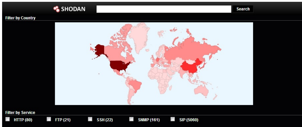
Figure 4. SHODAN interface
