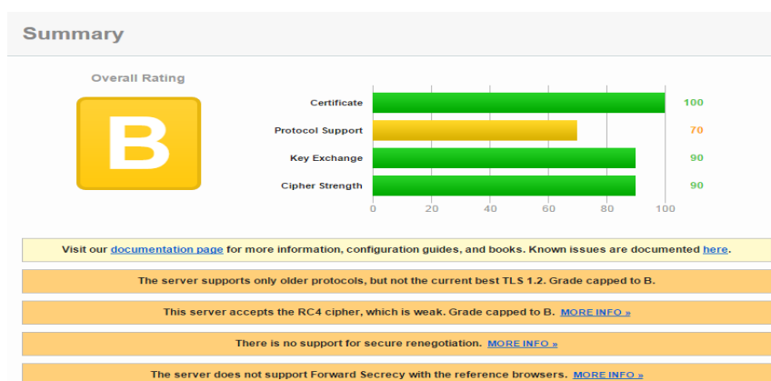
Figure 5. SSLyze run
