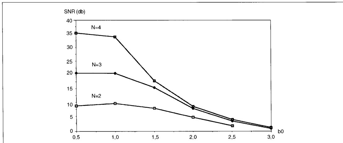
Fig. 8. Reconstruction Signal/Noise Ratio (SNR) error after frame decomposition for different sampling densities a_0 = 2^{1/N} ( N = number of voices per octave), b = a_0^k b_0 (after [DAU90a]). The basic wavelet is the Morlet wavelet (modulated Gaussian) used in [GRO89]. The reconstruction is done "as if" wavelets were orthogonal (see text), and its accuracy grows as N increases and b_0 decreases, i.e. as the density of the sampling grid of Fig. 7 increases. Therefore, redundancy refines the "orthogonal-like" reconstruction.
