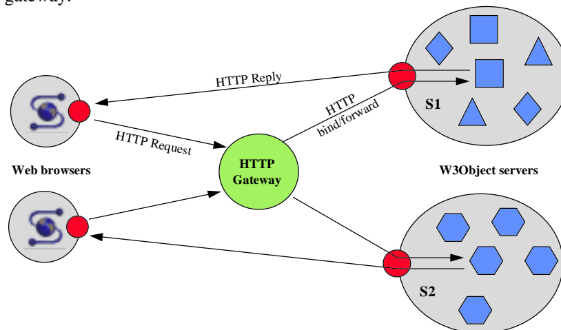
Figure 5: Client-object HTTP communication through gateway
