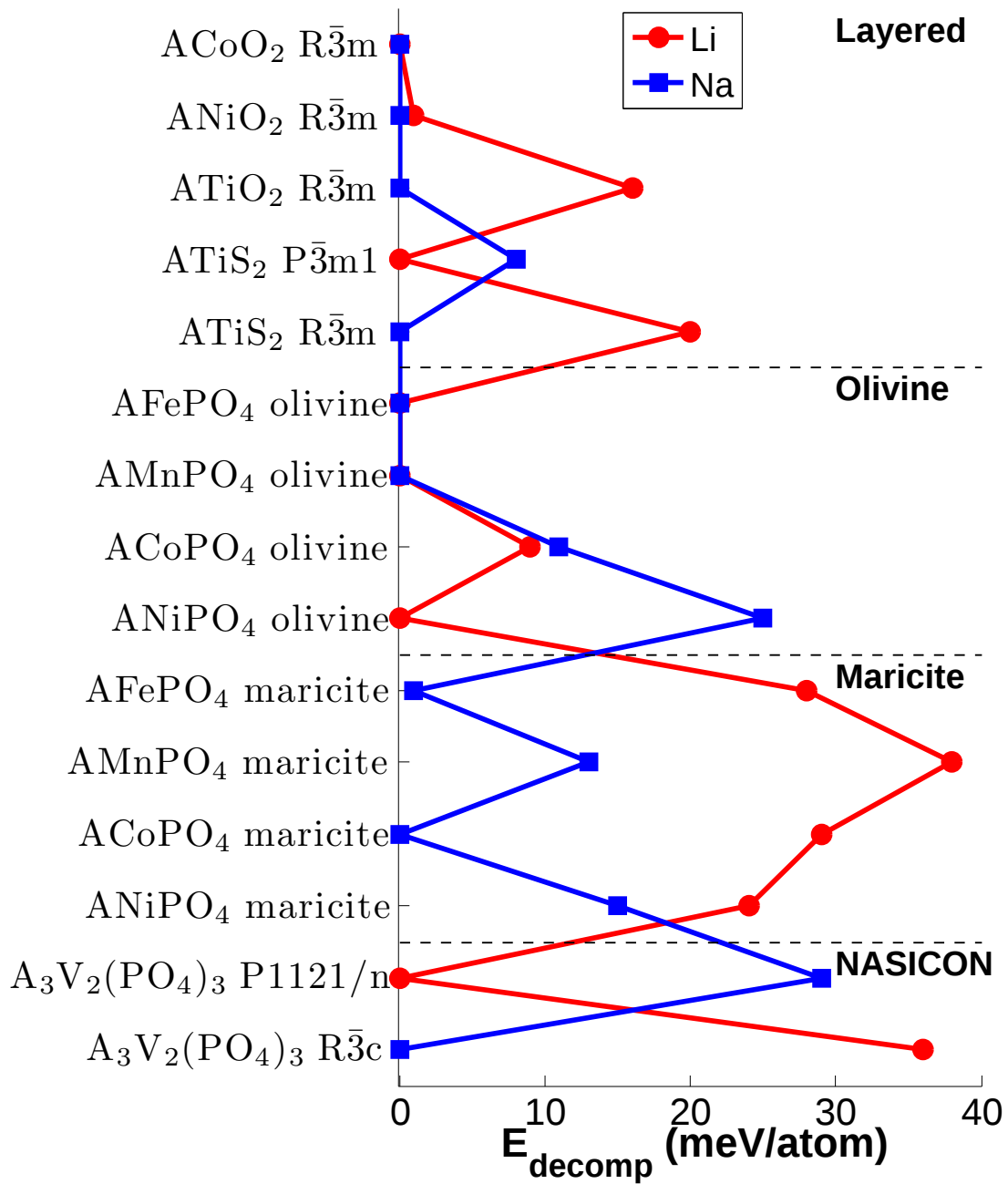
Figure 2: Calculated decomposition reaction energies per atom, E_{\text{decomp}} , for Na-ion and Li-ion battery compounds investigated. An E_{\text{decomp}} of 0 indicates that the structure is thermodynamically stable at 0 K.
