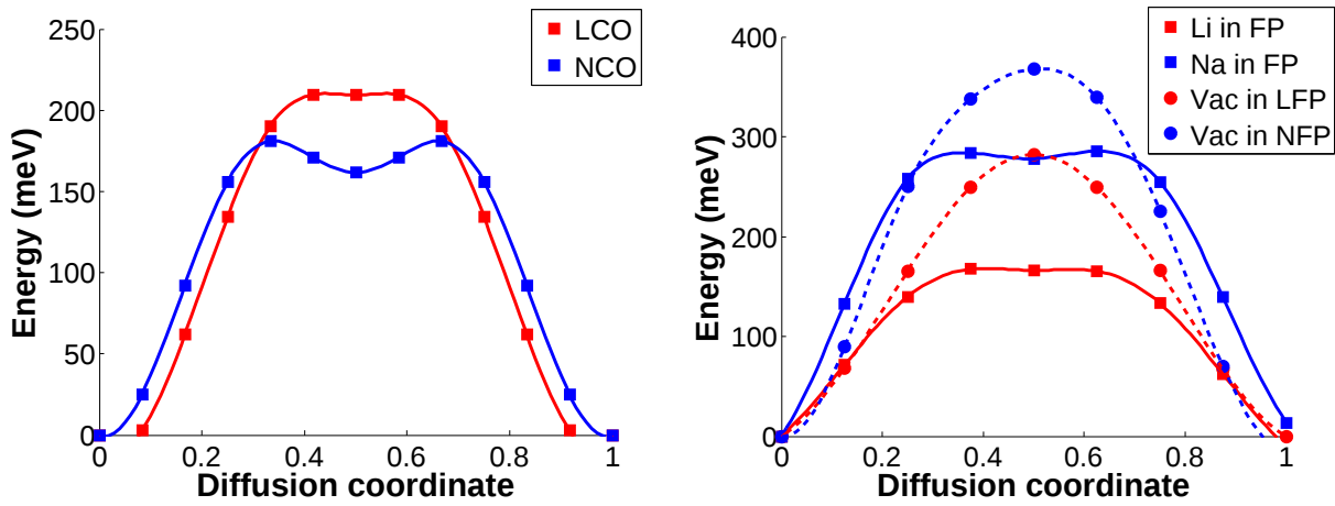
(a) Barrier for divacancy diffusion mechanism in layered \text{ACoO}_2 (b) Barriers for (i) alkali (A) diffusion in dealkaliated olivine \text{FePO}_4 (FP) and (ii) vacancy (V) diffusion in \text{AFePO}_4 (LFP and NFP)
