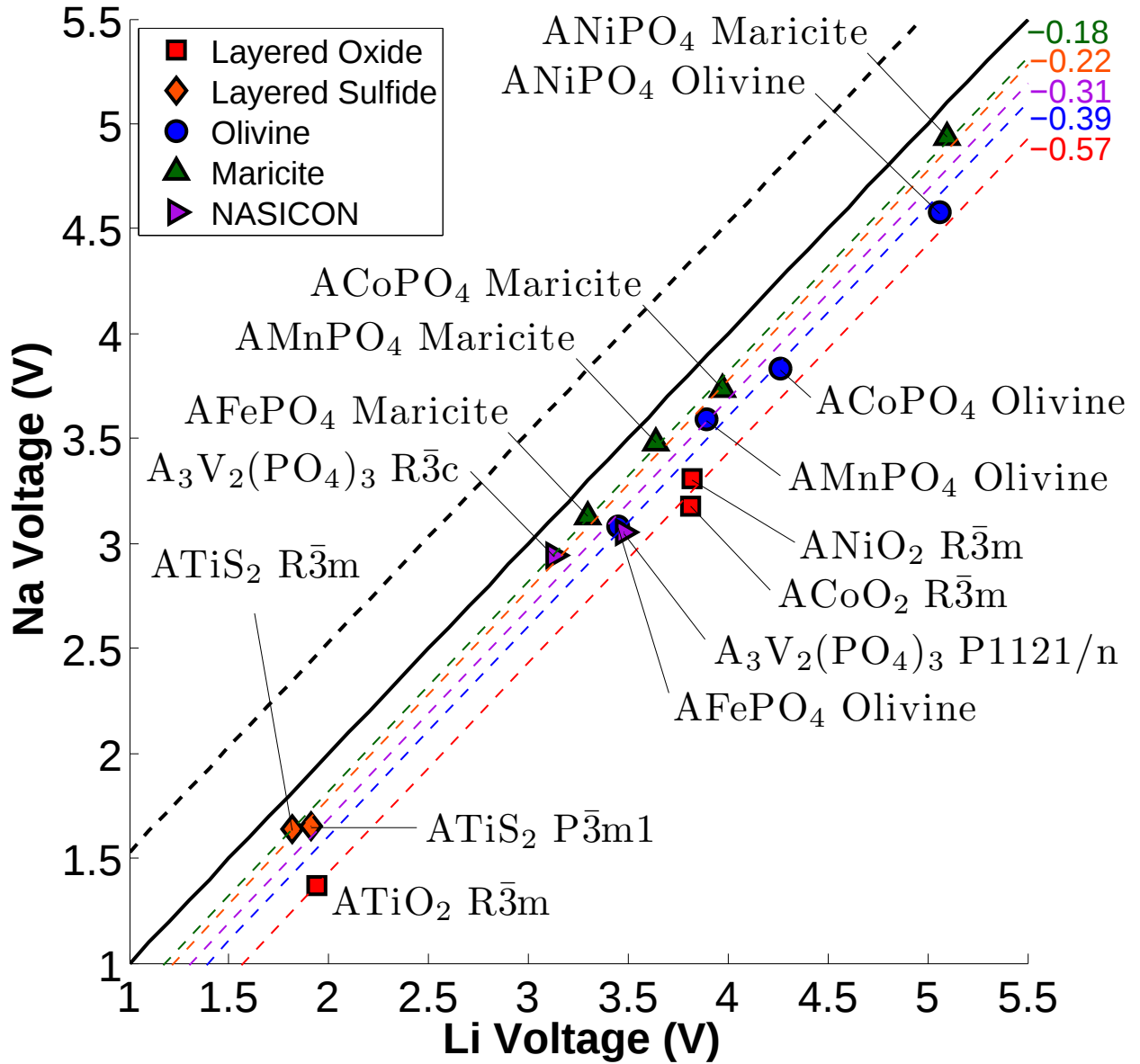
Figure 1: Calculated Na voltage vs calculated Li voltage for different structures. The black dashed line indicates the +0.53 V difference between the cohesive energies of Na and Li, while the other colored dashed lines indicate the fitted average voltage difference \Delta V_{\text{Na-Li}} .
