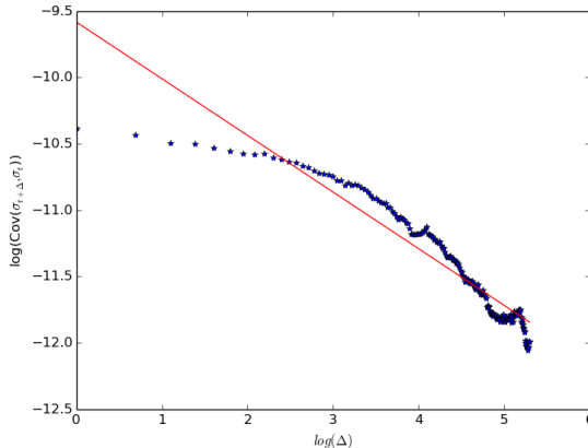
FIGURE : \log(\text{Cov}[\sigma_{x+\Delta}, \sigma_x]) as a function of \log(\Delta) . The autocorrelation function does not behave as a power law function.
