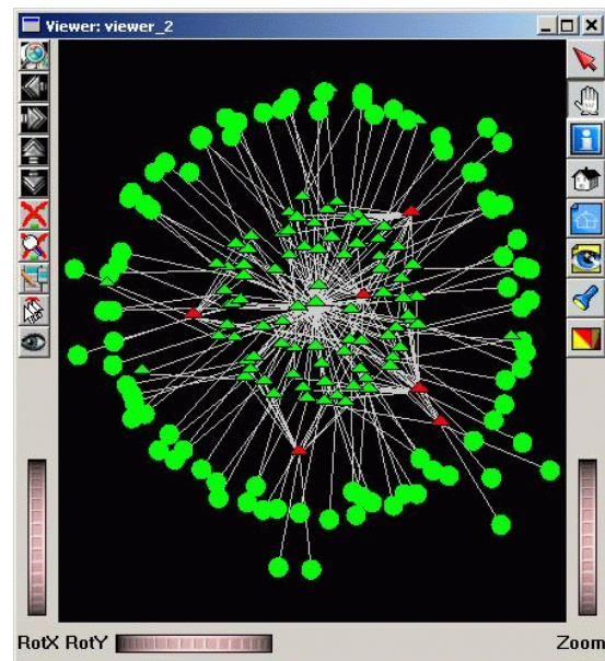
Figure 7. UAProf schema
