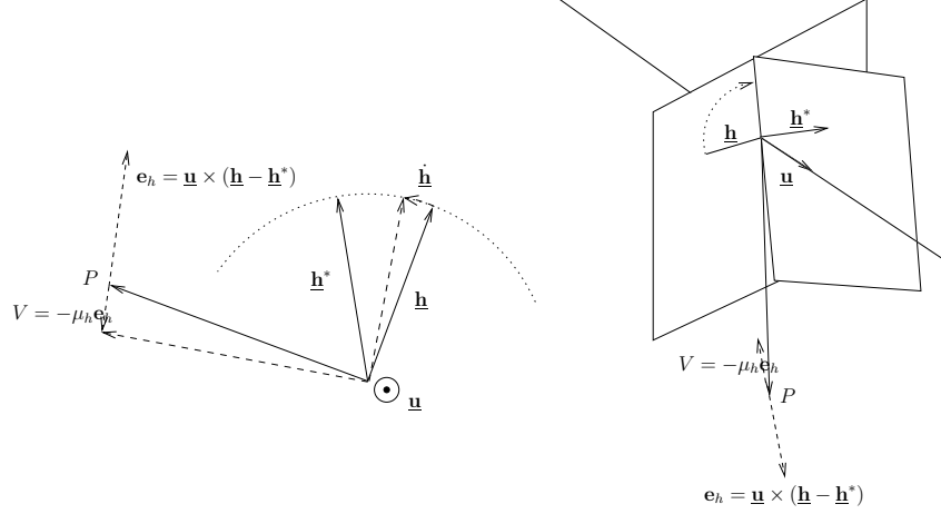
Figure 4: The action of the translation control V = -\mu_h \underline{\mathbf{u}} \times (\underline{\mathbf{h}} - \underline{\mathbf{h}}^*) : in the case where \underline{\mathbf{u}} = \underline{\mathbf{u}}^* (left) and in the general case (right).
