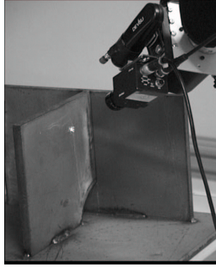
Figure 5: A laser pointer rigidly linked to the camera generates an epipolar line in the image.
