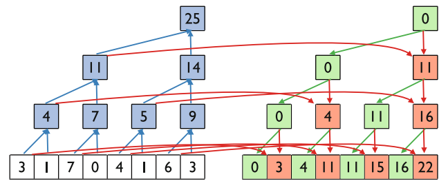
Fig. 1 Upsweep and downsweep phases of the prefix sum calculation, picture taken from [11]
