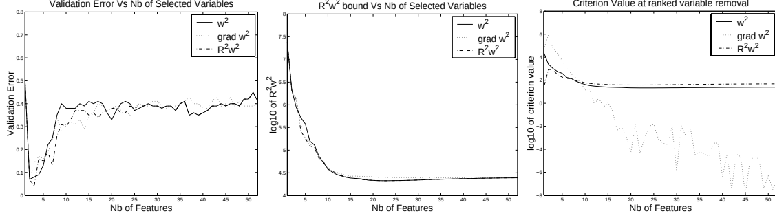
Figure 4: Different ways of choosing the number of ranked features to be provided to the predictor. Results for \|w\|^2 , \nabla\|w\|^2 and R^2 w^2 are depicted. (left) Validation error. (middle) L error Estimation with \frac{1}{m}R^2 w^2 . (right) Criterion value when variable has been removed.
