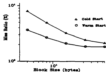
Fig. 4. Miss Ratio vs. Block Size for warm and cold starts; VAX-11 traces.
