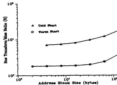
Fig. 7. Miss ratio vs. Address Block Size for warm and cold starts.
