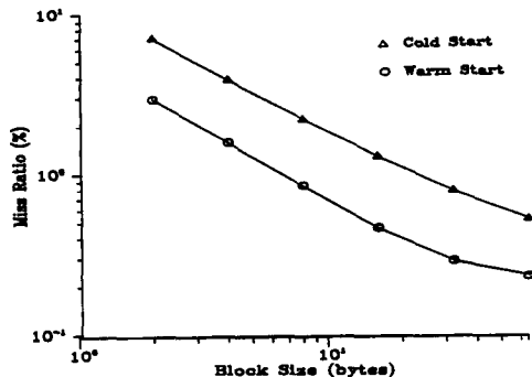
Fig. 3. Miss Ratio vs. Block Size for warm and cold starts; PDP-11 traces.
