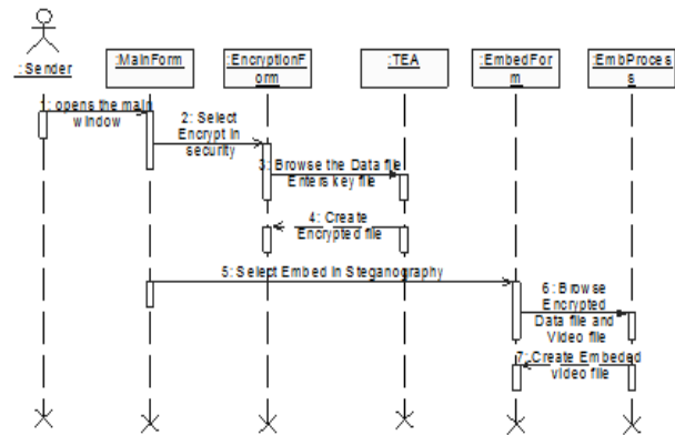
Fig. 4: Sequence diagram for Sender
