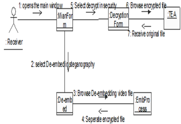
Fig. 7: Collaboration diagram for Receiver
