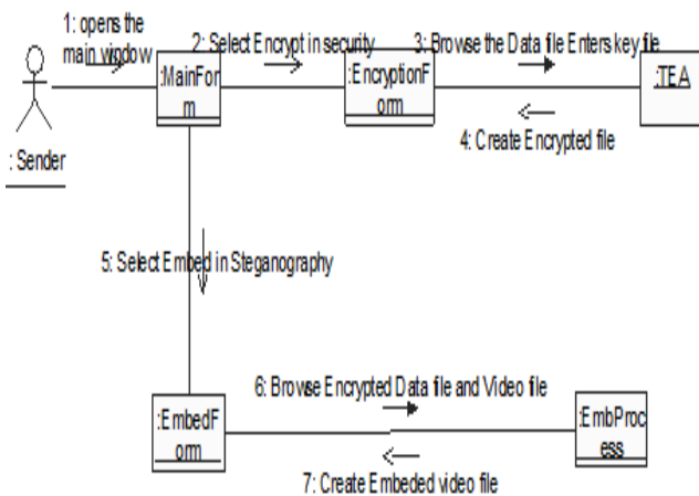
Fig. 6: Collaboration diagram for Sender
