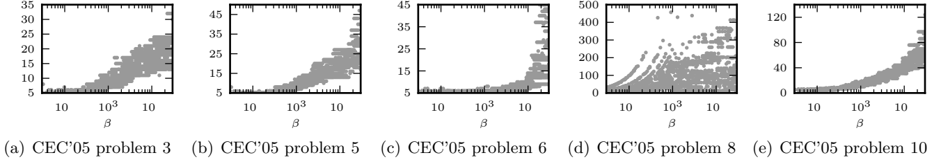
Figure 6: Scatter plots of the combined results from all of tMOPSO’s independent tuning runs, showing the optimal population size versus the OFE budget available. Each sub figure shows the results for DE tuned to a different CEC’05 optimization problem.
