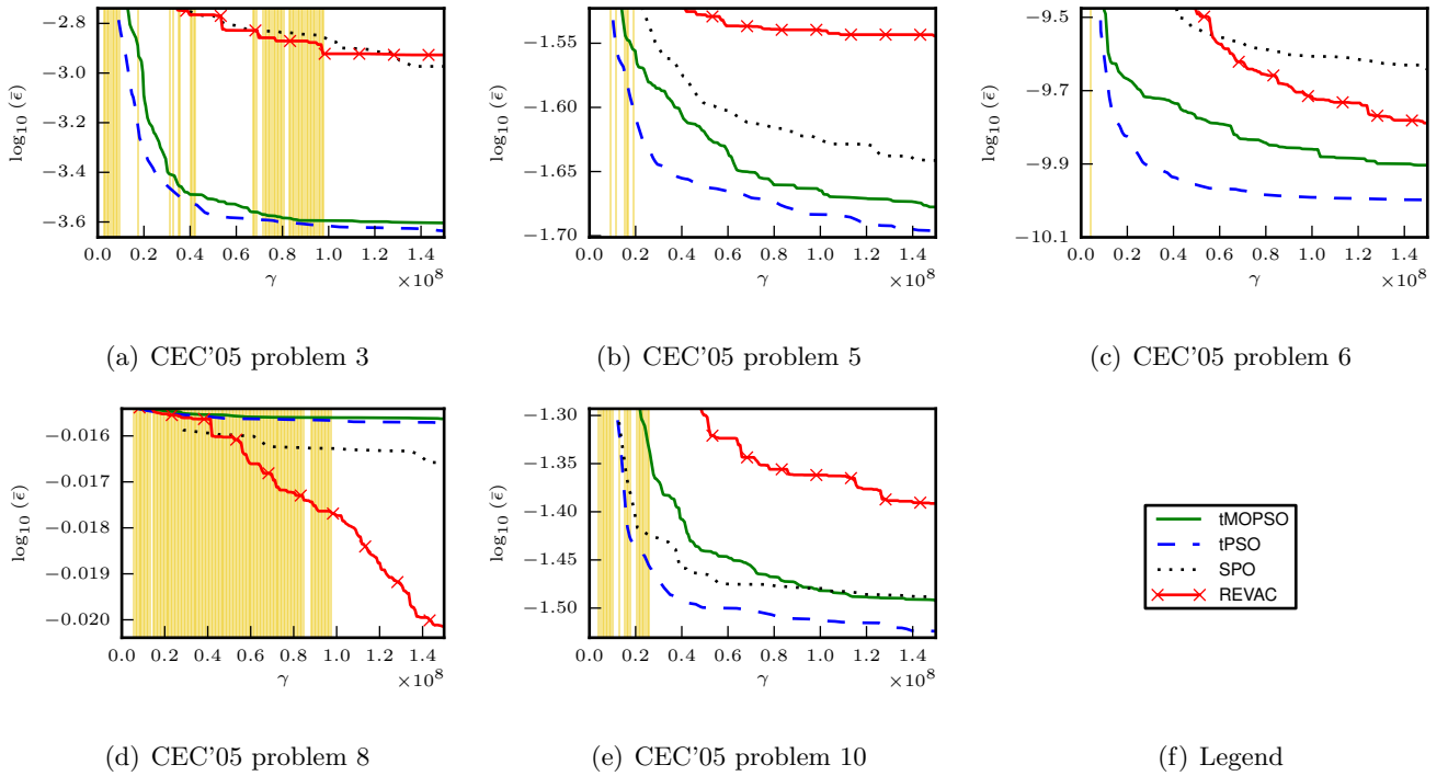
Figure 4: Best mean minimum solution error ( \bar{\epsilon} ) versus the number of application layer evaluations made ( \gamma ) of the multi-objective tuning algorithms, applied to the DE tuning problems. Shaded regions indicate \gamma where a Mann-Whitney U-test failed to show with a confidence level of 95% that the leading sample mean is better than the other sample means.
