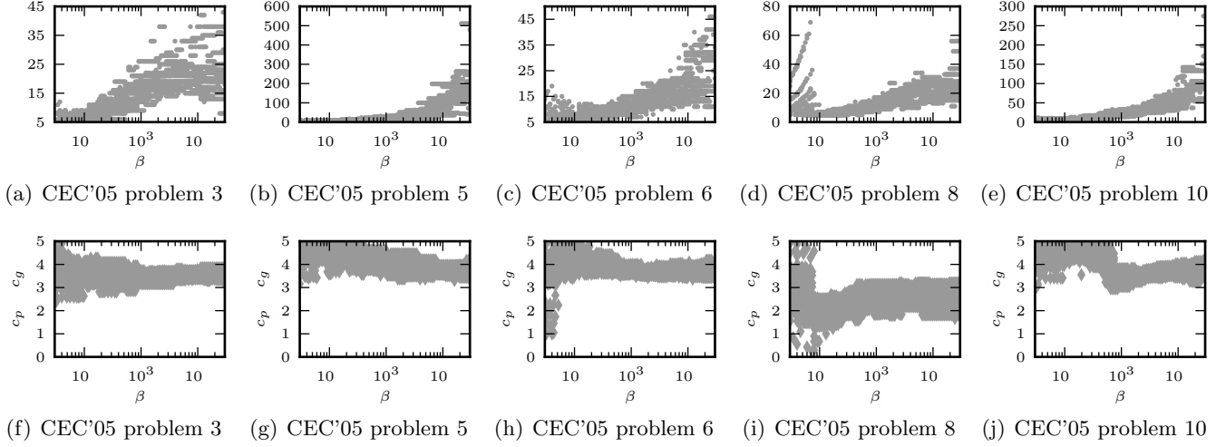
Figure 7: Scatter plots of the combined results from all of tMOPSO’s independent tuning runs, showing the optimal swarm size and acceleration constant sum versus the OFE budget available. Each sub figure shows the results for PSO tuned to a different CEC’05 optimization problem.
