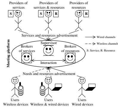
Figure 1: Framework architecture
