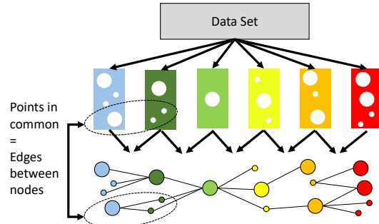
Figure 3. General Concept of TDA as implemented in the Mapper algorithm, adapted from [34]
