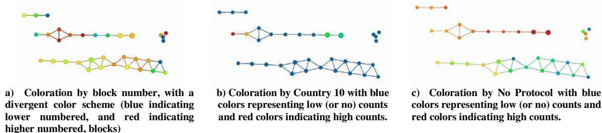
Figure 10. Custom topological model using Metric: Cosine, Lens 1: Approximate Kurtosis, Lens 2: Variance. Resolution: 30 (both lenses), gain: 2.50 (both lenses), with neither lens equalized.
