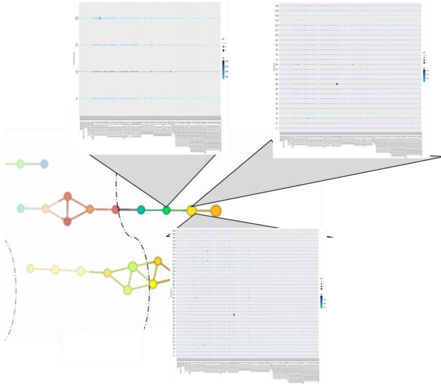
Figure 11. Topological Model from Figure 10a with incorporated HMAT visualizations for selected nodes.
