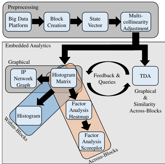
Figure 4. Multivariate and Graphical Approach to Firewall Log Anomaly Detection, extended from [3], to include the feedback and TDA for log analysis
