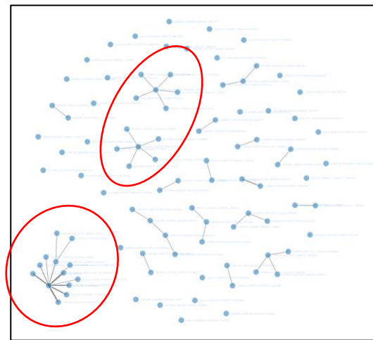
Figure 9. IP Network Graph of Block 14 with detected port scan
