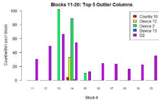
Figure 6. Block 14 Within-Blocks Analysis with Top 5 Anomalous Columns per Breakdown Distance
