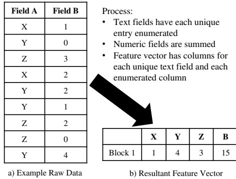
Figure 2. Generic feature vector creation process: (a) raw data; (b) resultant feature vector, from [3]
