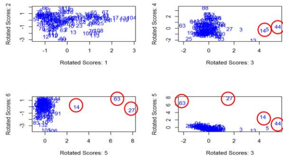
Figure 8. Factor plot using varimax rotated FA scores and identified outlier blocks
