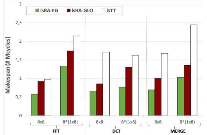
Fig. 13: Makespan comparison of sequential execution (8x8) and eight executions of the parallel execution (8*(1x8))
