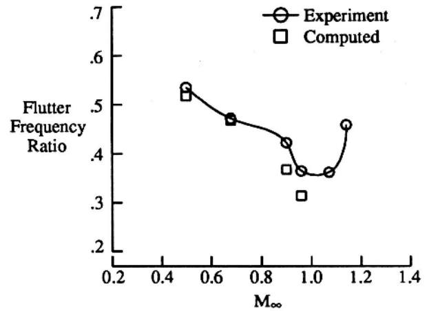
(b) Flutter frequency ratio.
