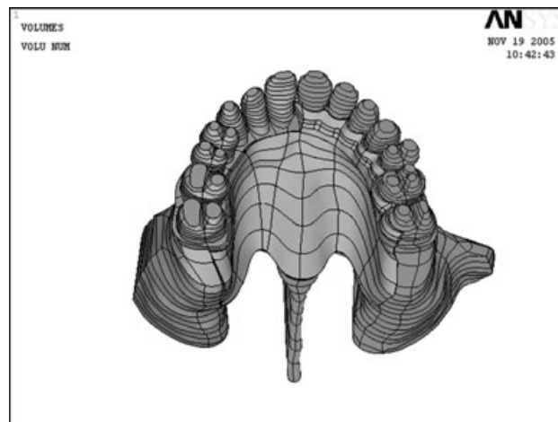
Fig. 3. 3D FEM of the obturator prostheses with casting palatal plate.
