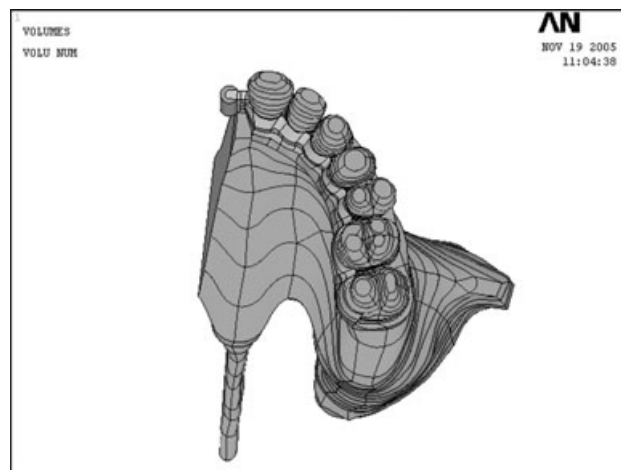
Fig. 2. 3D FEM of the lingual guide plane on all the remaining teeth (from central incisor to second molar) with attachment on the mesial surface of the central incisor.
