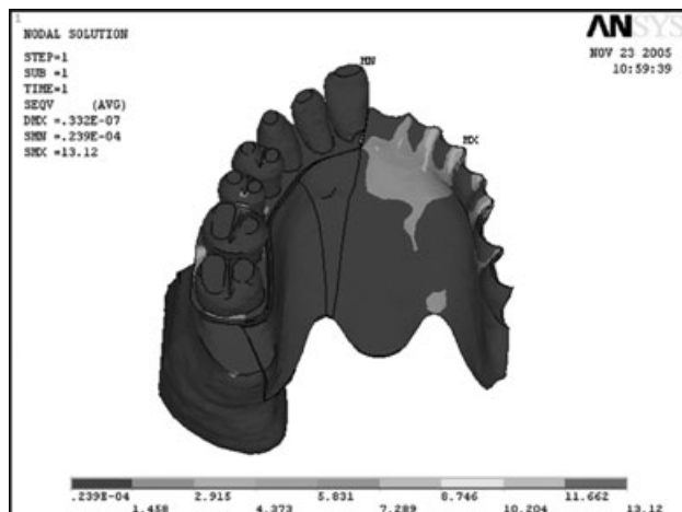
Fig. 4. Stress on the prostheses (model 1).
