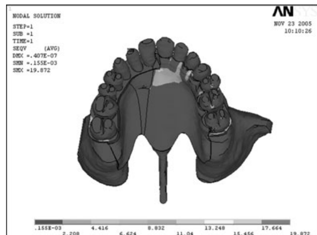
Fig. 7. Stress on the prostheses with attachment (model 2).
