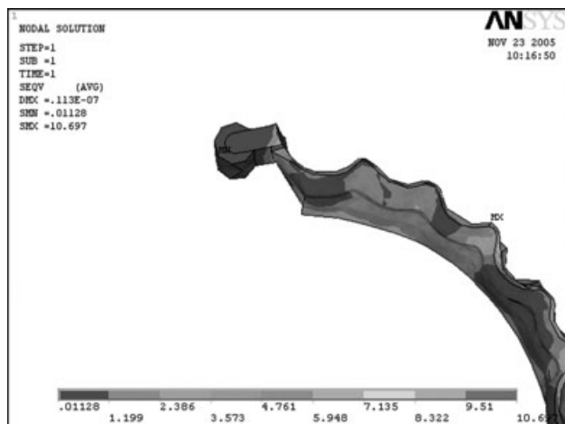
Fig. 10. Stress on the lingual guide plane with attachment.
