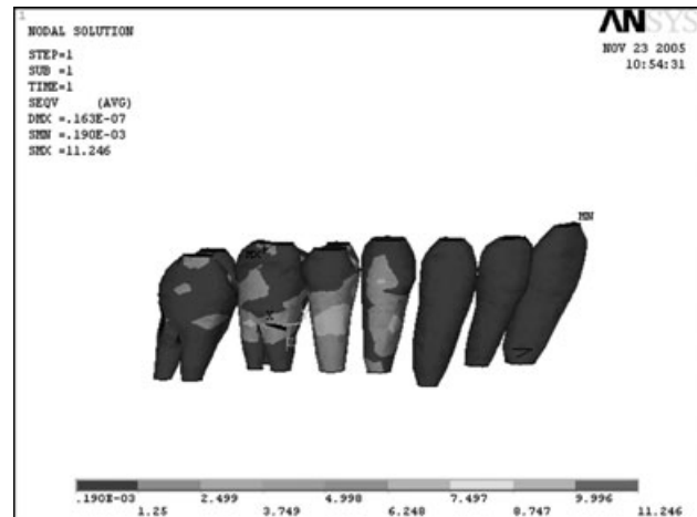
Fig. 5. Stress on the remaining teeth (model 1).
