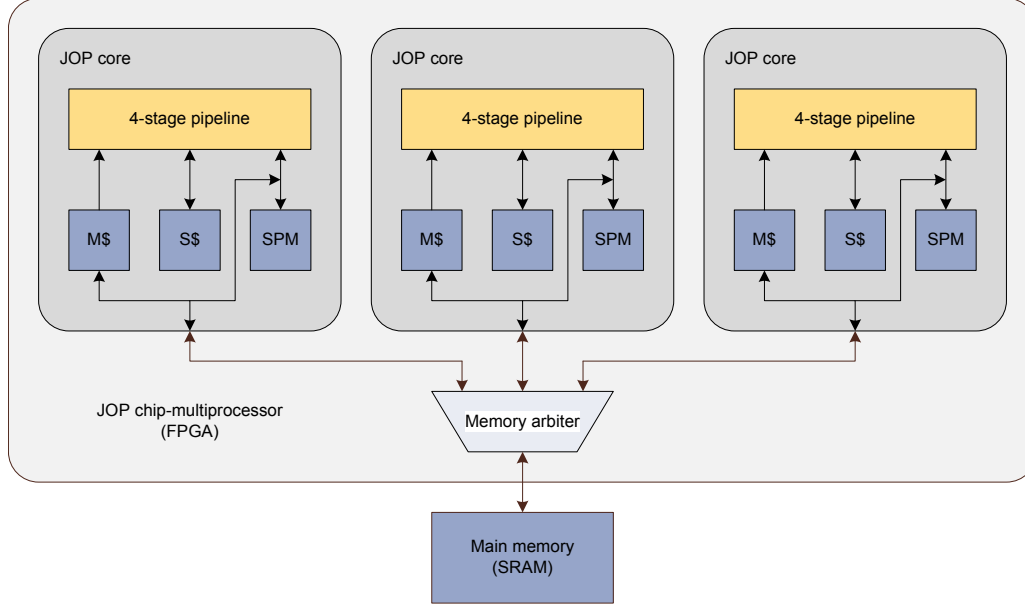
Figure 2. A three core JOP CMP system with three core-local memory areas
