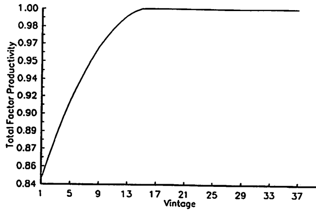
Figure 2 Learning Curve
