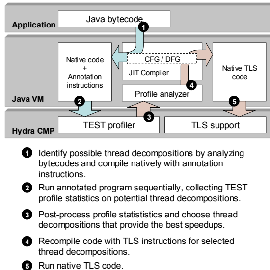
Figure 1 – Block diagram of Jrpm.
