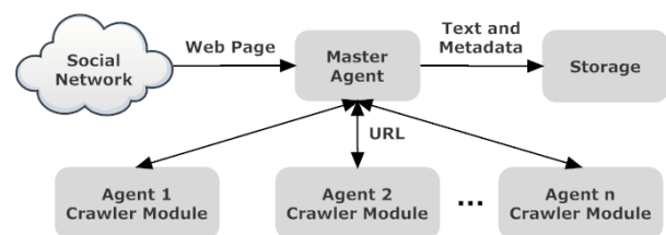
Fig. 3: Distributed web crawling.
