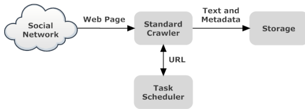
Fig. 1: Architecture of crawler.
