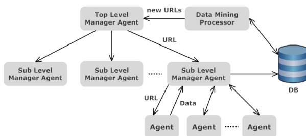
Fig. 5: System concept overview.
