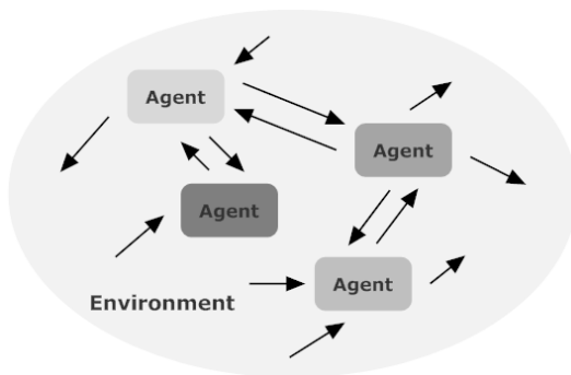
Fig. 2: Multi-agent system.
