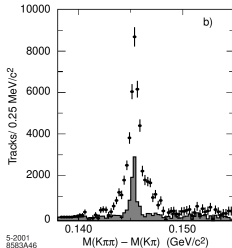
Figure 41. Reconstruction of low momentum tracks: the mass difference, \Delta M = M(K^- \pi^+ \pi^+) - M(K^- \pi^+) , both for all detected events (data points) and for events in which the low momentum pion is reconstructed both in the SVT and DCH (histogram). Backgrounds from combinatorics and fake tracks, as well as non-resonant data have been subtracted.
