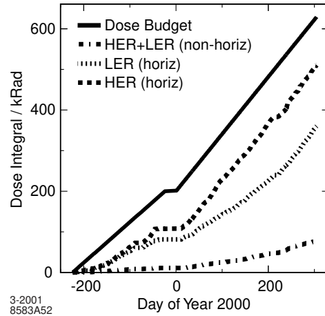
Figure 7. The integrated radiation dose as measured by PIN diodes located at three different positions, showing contributions from the HER ( \phi = 180^\circ ), and the LER ( \phi = 0^\circ ) in the horizontal plane, and from both beams combined elsewhere. Also shown is the SVT radiation budget for the first 500 days of operation.
