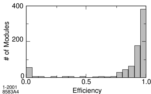
Figure 76. Distribution of the efficiency for all RPC modules measured with cosmic rays in June 1999. Some 50 modules were not operational at that time.
