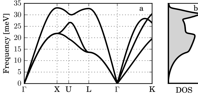
Figure 9: Continuum of vibrational states for bulk FCC aluminum. a) Phonon band structure calculated with a 7 \times 7 \times 7 supercell using effective medium theory, i.e. the EMT calculator in ASE. b) The phonon density of states for the same system, integrated over an equispaced 50 \times 50 \times 50 grid.
