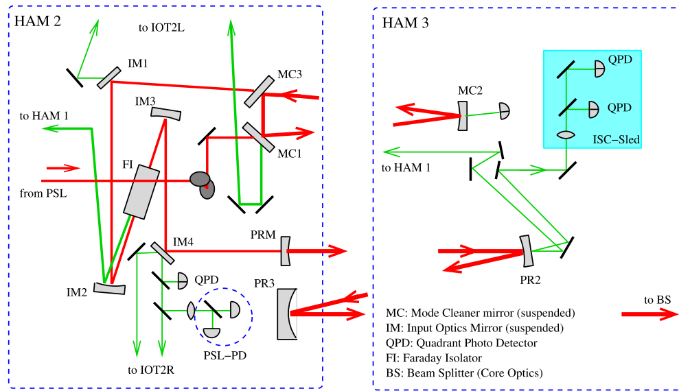
FIG. 4. A sketch of the in-vacuum components and beam directions within the input optics in HAM 2 and HAM 3. The red beam is the forward going main beam while the green beams are auxiliary beams. The main items in the in-vacuum input optics are the input mode cleaner (IMC) which is formed by the three mirrors MC1, MC2, and MC3; the Faraday isolator (FI); and the four suspended steering mirrors IM1-4 of which IM2 and 3 match the spatial mode of the IMC into the main interferometer. The recycling cavity mirrors PRM, PR2, and PR3 are not part of the input optics. The ISC sled in HAM3 belongs to the interferometer sensing and control subsystem and provides alignment signals for the recycling cavity.
