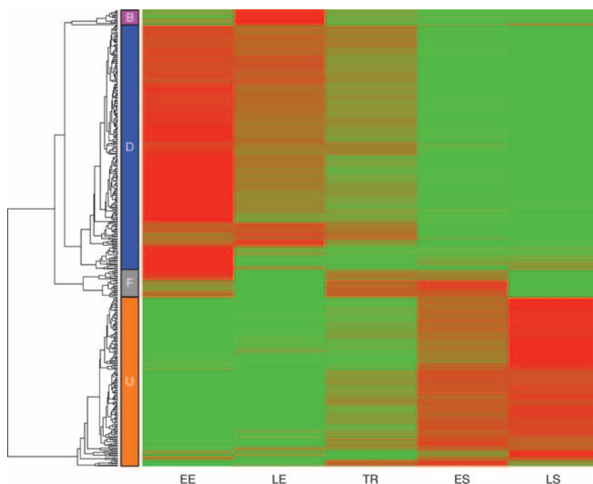
FIG. 2. Hierarchical clustering and dendrogram of 415 differentially expressed genes ( >2 -fold; false discovery rate, <0.01 ). The color gradient from green to red represents increasing microarray hybridization intensity. Four major response groups were detected and are identified by the colored boxes labeled B (biphasic), D (down-regulated), F (fluctuating), and U (up-regulated).
