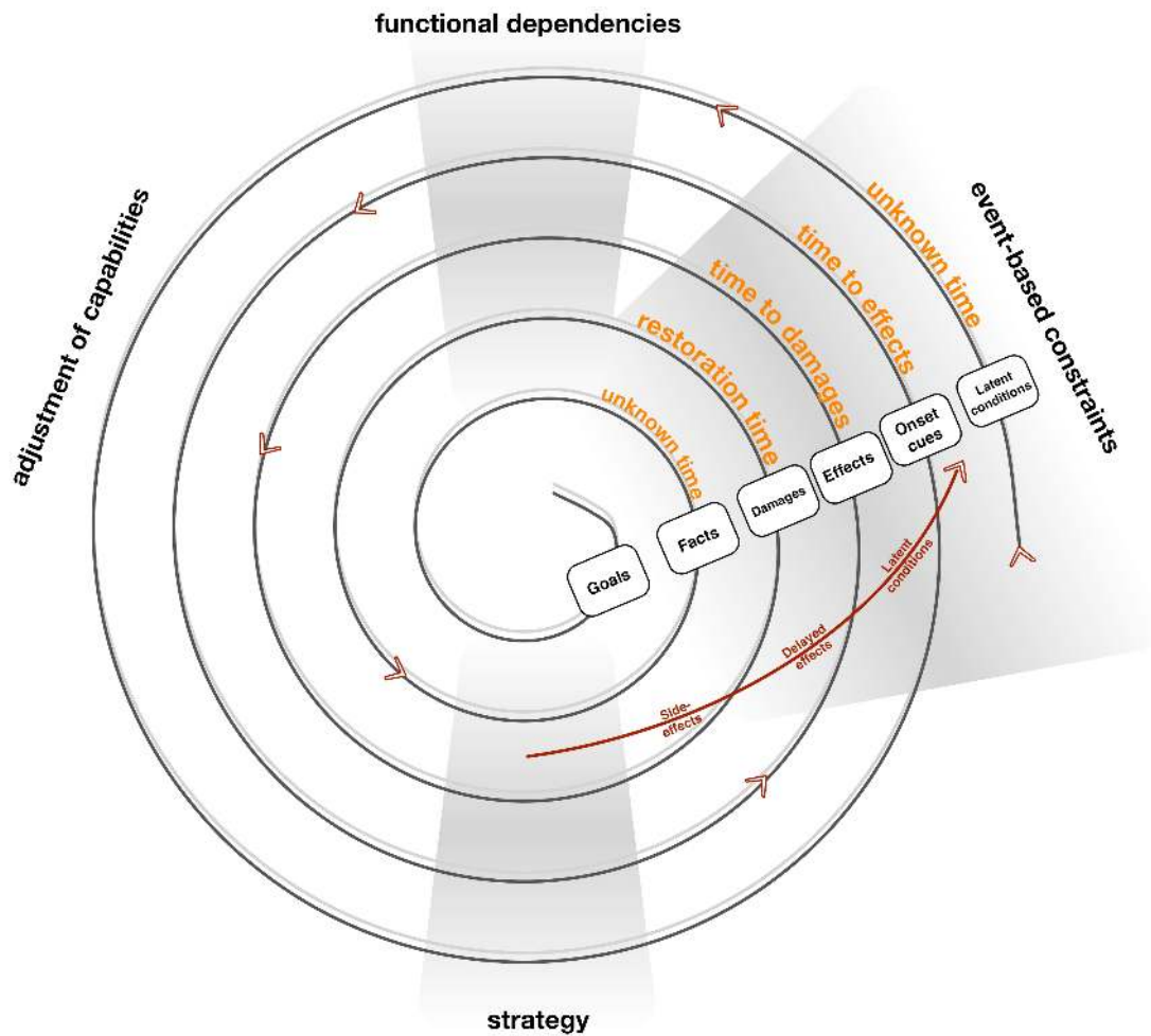
Figure 1. Event-based constraints.
