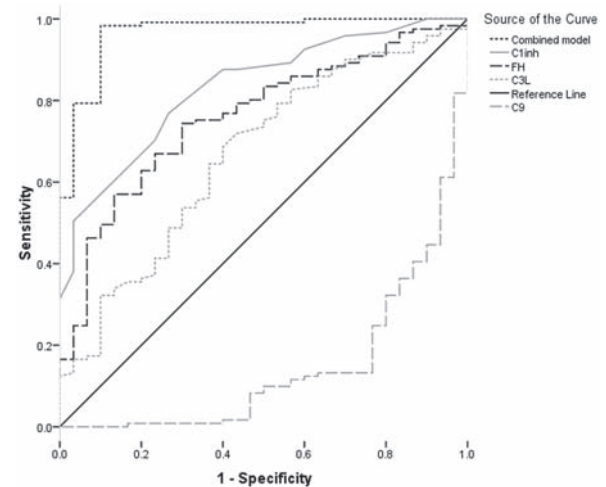
Figure 2. Receiver operating characteristic (ROC) curve to predict the probability of MS compared to control subjects. Combined model C statistic 0.97. For the individual components of the model; C3 C statistic 0.67, C9 C statistic 0.14, C1inh C statistic 0.83 and FH C statistic 0.76.
