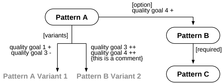
Figure 2. Example of a pattern sequence diagram
