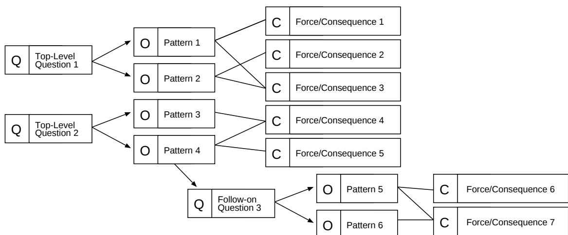
Figure 3. Activities for mapping patterns to a design space
