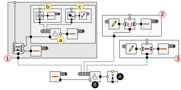
Figure 4: Instantiating a mutator for a list.
