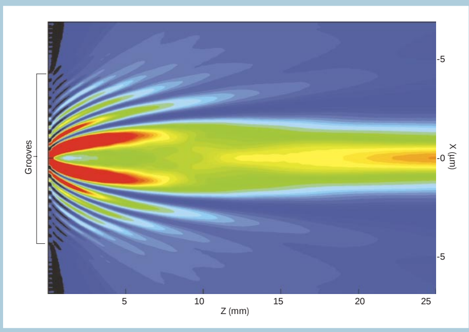
Figure 5 Calculated pattern of light emerging from a single slit surrounded by a finite array of grooves (courtesy of F. J. García-Vidal, Universidad Autónoma de Madrid, Spain) and L. Martín-Moreno (Universidad de Zaragoza, Spain). For this simulation there were 10 grooves on each side of the slit, each of width 40 nm and depth 100 nm. The groove period was 500 nm. The contour plot shows the spatial dependence of the component of the Poynting vector along the radial direction for a wavelength of 560 nm, corresponding to a spectral transmission maximum. Blue indicates low intensity ( 3 \times 10^{-4} ), and red high (1).
