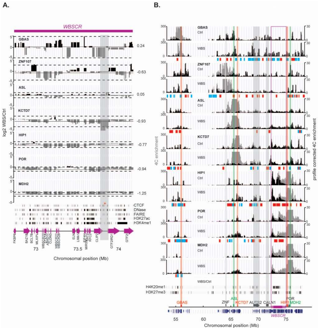
Figure 2. Modification of short-range interactions in WBS compared to control cells. (A) Close-up of the log 2 -fold interaction changes in WBS versus Ctrl within the WBSR. The black line indicates the median of the changes within the WBSR, which is also displayed at the right of each graph. The dashed lines show the 95% confidence interval. The positions of all genes are displayed at the bottom with purple arrows. The area highlighted in grey pinpoints the higher interactions in Ctrl cells between the KCTD7 viewpoint and the region around the CLIP2 and GTF2IRD1 genes. The black ticks below show the location of the five marks of regulatory regions in GM12878 cells (as found in the ENCODE data), including CTCF binding sites, DHSs, FAIRE sites, H3K27ac and H3K4me1 and binding sites, with one overlapping mark highlighted with a red asterisk. (B) Windowed 4C signal of each of the seven viewpoints in both Ctrl and WBS cells around the WBSR (see the legend of Figure 1B for details about the structures outlined). The log 2 -fold change of the windowed 4C data in WBS over control cells was calculated, and the resulting positive or negative Bricks are indicated below each viewpoint graphs, by blue or red bars, respectively. The significant changes in histone marks (as defined by SICER) are plotted below by ticks.
