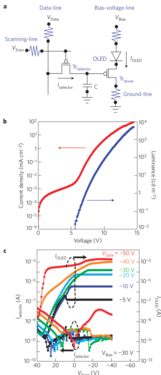
Figure 3 | Stretchable display cells comprising an organic LED and a 2T1C driving cell. a , Circuit diagram of one stretchable display cell comprising an organic LED and a 2T1C driving cell. I_{\text{selector}} and I_{\text{OLED}} represent currents passing through the selector transistor \text{Tr}_{\text{selector}} and through the organic LED, respectively. Display cells are interconnected with each other through printed elastic conductors that work as scanning-, data-, bias-voltage- and ground-lines. V_{\text{Scan}} , V_{\text{Data}} and V_{\text{Bias}} represent voltages applied to scanning-, data- and bias-voltage-lines, respectively. The capacitance of the circuit ( C ) is 215 pF. The resistor symbols represent printed elastic conductors.
