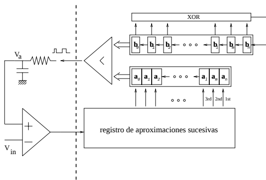
Figure 3: Analog to stochastic conversion
