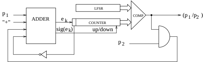
Figure 7: Stochastic division circuit
