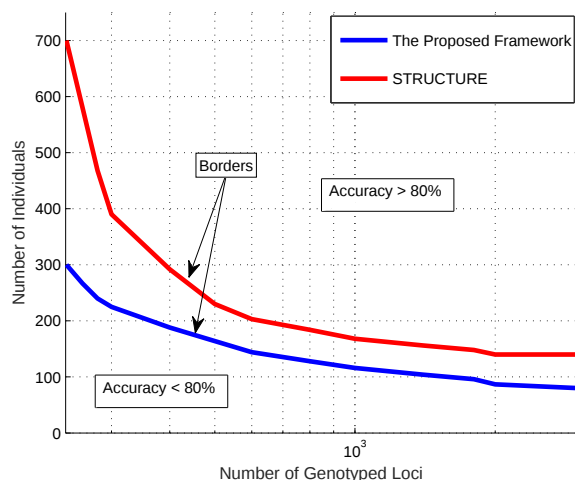
Fig. 4. The area in N - L plane (number of individuals and number of genotyped loci) in which the accuracy of clustering methods are above 80% in a two-class problem. The proposed method is compared with the STRUCTURE framework. It can be seen that our method has an acceptable performance in a relatively larger area of the plane, implying a more robust performance for small size datasets. The achieved improvement is due to employing disease infection labels during the clustering.
