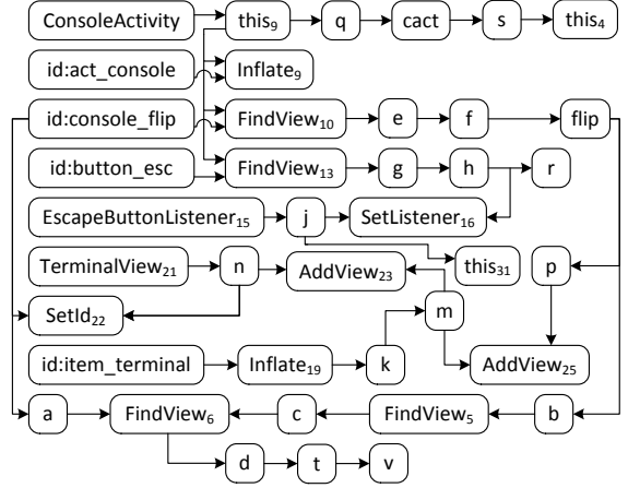
Figure 3: Partial constraint graph for the running example.
