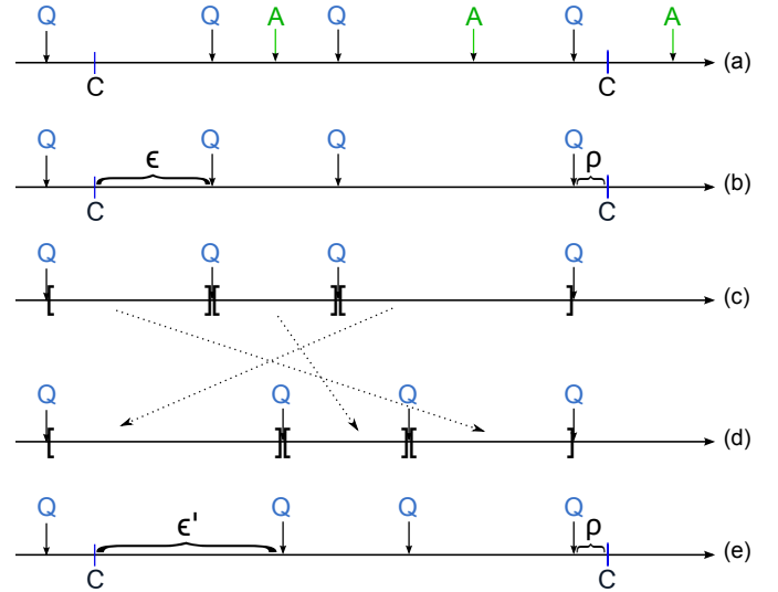
Fig. 4: The steps to generate a simulated time-series of StackOverflow activities.
