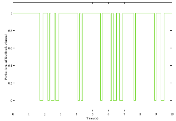
FIGURE 7. Distribution of \alpha_k .
