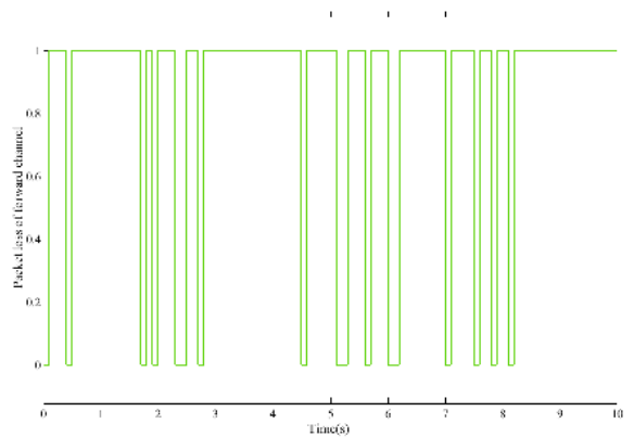
FIGURE 8. Distribution of \beta_k .
