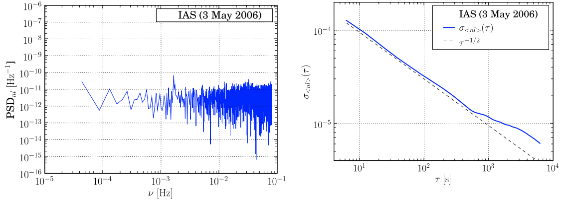
Figure 3. Left: power spectrum density of the nulling function, PSD_{nl} . Note that 1/f component is negligible. Right: standard deviations of the running average of the nulling function over the time interval \tau , \sigma_{<nl>}(\tau) (curve above). A (displaced) \tau^{-1/2} function is shown for comparison (line below). Note that up to \tau \approx 500 s, the experimental curve is consistent with the \tau^{-1/2} behaviour, with \sigma_{<nl>}(500 \text{ s}) \approx 1.5 \times 10^{-5} .
