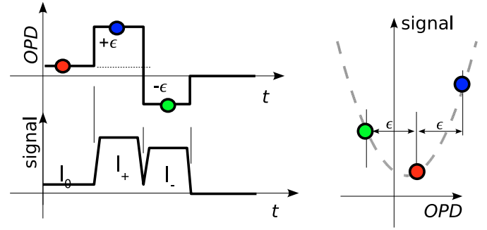
Figure 1. OPD dithering cycle. The top curve shows schematically the position of the delay line whereas the bottom curve is an idealised representation of the corresponding detected signal. From an initial position the dithering alters the OPD value by +\epsilon(\text{OPD}) with respect to the initial position. A measurement of the flux is performed. During the next stage, the dithering algorithm again alters the OPD, this time by -\epsilon(\text{OPD}) with respect to the initial position. Another measurement is performed. We thus know three points, defining a parabola ( right ), which allows us to calculate and reach a new working position of the OPD (the vertex of the parabola).
