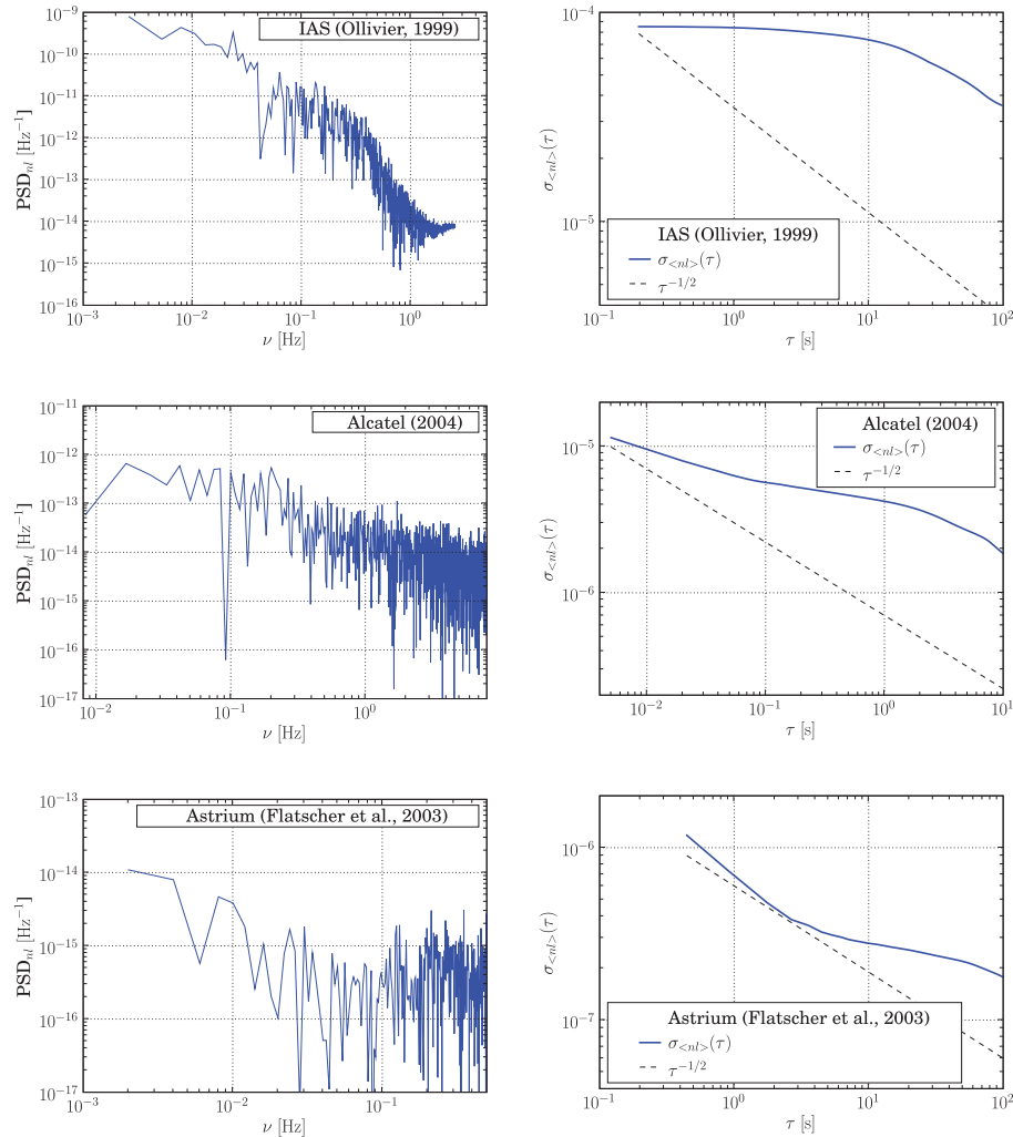
Figure 4. Comparison with three other experiments. Left column: power spectrum distributions. Right column: standard deviation of the running average of nl over time \tau , \sigma_{<nl>}(\tau) . Top: results from the nulling experiment Ollivier (1999); Ollivier et al. (2001). The increase in the PSD for low values of \nu is clear. In the range of 0.3–0.01 Hz the PSD is approximately \nu^{-1.35} , a behaviour close to the “classical” 1/f \equiv 1/\nu behaviour. In the frequency range investigated by that experiment, \sigma decreases with \tau but more slowly than \tau^{-1/2} , which is typical of PSDs with 1/f -like components. Centre: results from the nulling experiment by Alcatel (2004), using a laser diode at \sim 1.57 \mu\text{m} and an integrated optics recombiner. The increase of the PSD at low frequencies is clear. From 0.1 to 1 Hz the curve goes approximately as 1/\nu (courtesy Alcatel Space Industry). Bottom: results obtained by Flatscher et al. (2003). The duration of the experiment is the longest of the three. The null curve between 1000 and 1500 s is selected (Chazelas et al. 2006) to compute the PSD because it has the best qualities. A low-frequency increase in the PSD is present. From 0.01 to 0.1 Hz it is approximately 1/\nu (courtesy Astrium, Germany).
