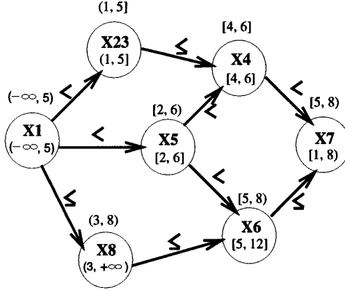
Fig. 2. Construction of assignment satisfying G_S in the real domain.
