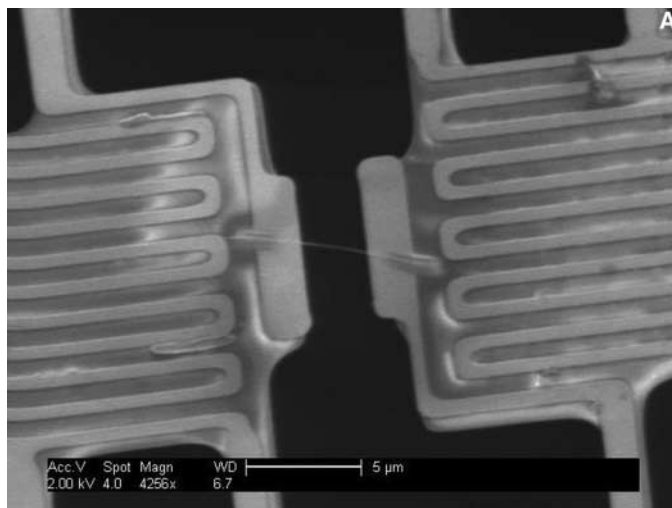
Fig. 2. (A) The SEM image of a CNT (light gray line in center) connected to the electrodes. Scale bar, 5 \mu\text{m} . (B and C) The corresponding low-magnification TEM images of the same CNT in (A), before (B) and after (C) \text{C}_9\text{H}_{16}\text{Pt} was deposited.
