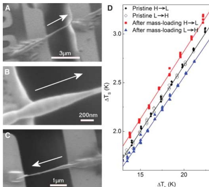
Fig. 3. (A to C) SEM images of three different BNNTs after deposition of C_9H_{16}Pt . The rectification measured was 7, 4, and 3%. The arrows denote the direction of heat flow, indicating where the thermal conductance is higher than that of the opposite direction. (D) Graphical representation of \Delta T_h and \Delta T_s for the BNNT in (A) before and after deposition of C_9H_{16}Pt . The solid lines are best-fit slopes intersecting the origin. For clarity, only data collected over a limited range of \Delta T_h and \Delta T_s are shown; data of similar quality were obtained over a much wider range of \Delta T_h and \Delta T_s .
