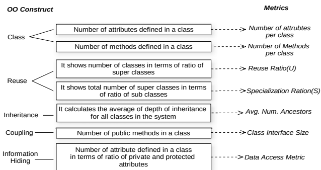
Fig 2 QMOOD Metrics
