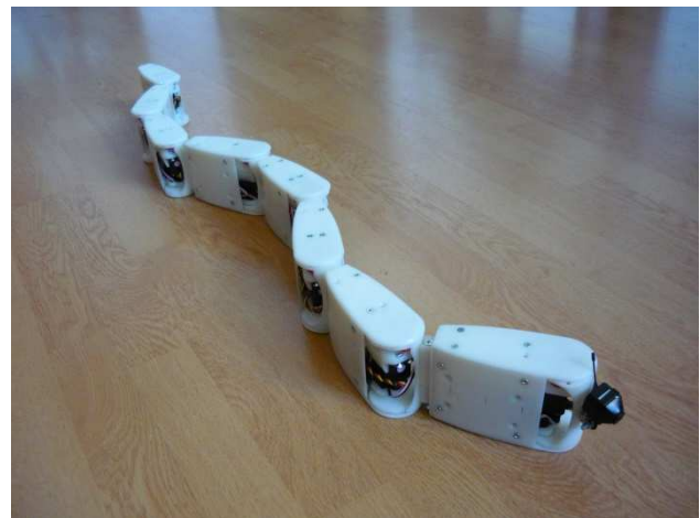
Figure 9 Realisation of snake-like robot “Locosnake”
