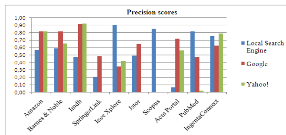
Fig.1 Precision scores of site-specific search engines, Google and Yahoo!
