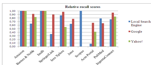
Fig.2 Relative recall scores of site-specific search engines, Google and Yahoo!
