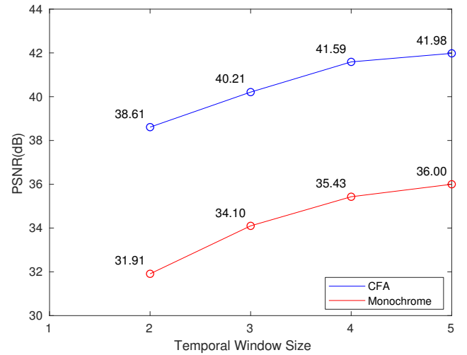
Figure 10: The effect of temporal window size, \beta , on the reconstruction quality of the Boxer-Gladiator-Irish data set for both designs using a monochrome sensor and a CFA-equipped sensor.
