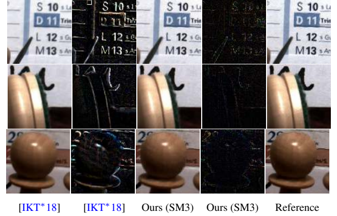
Figure 9: Visual comparison of our method using SM3 versus Inagaki et al. [IKT*18] for three data sets: Boxer-Gladiator-Irish , Chess , and Chess-moving ; shown from top to bottom, respectively. For quantitative results see tables 2 and 3. Error insets have a 5x intensity scaling to facilitate comparisons.
