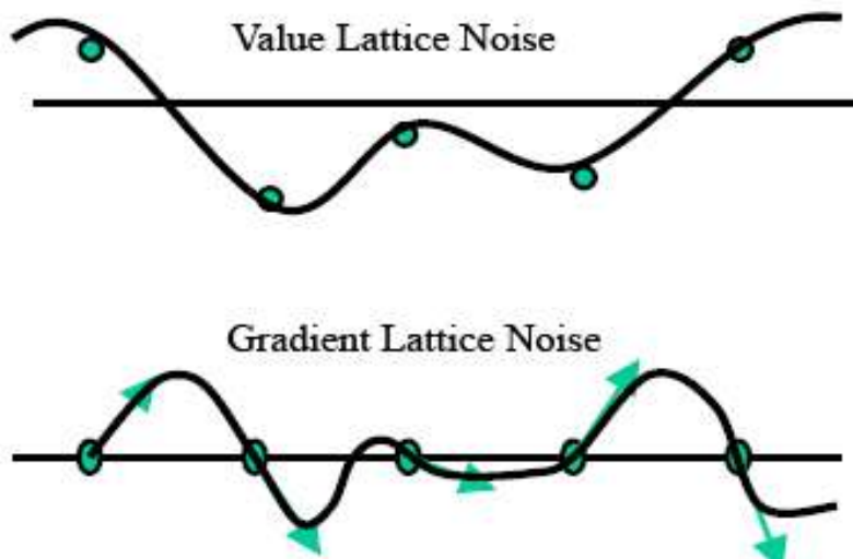
Figure 1. 1D Noise Functions
