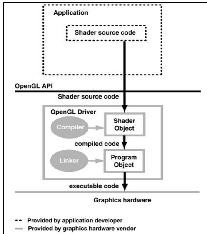
Figure 10. Execution Model for OpenGL Shaders (From: OpenGL Shading Language Book)
