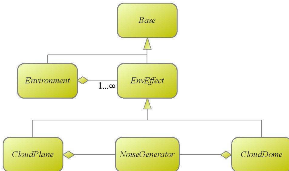
Figure 3. Class Hierarchy
