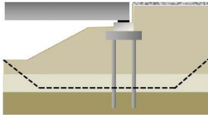
Figure 2-6: Shear failure surface near bridge abutment (after Caltrans 2013)
