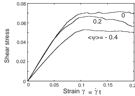
FIG. 10. Stress-strain curves in two-phase states with \langle \psi \rangle = -0.4, 0 , and 0.2 . There are no initial dislocations. Yield occurs with dislocation formation.
