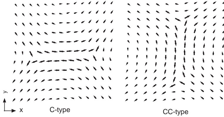
FIG. 2. Displacement \mathbf{u} around type C and type CC slips in the most favorable orientation in shear strain. The arrows are from the original undeformed position to the displaced position.
