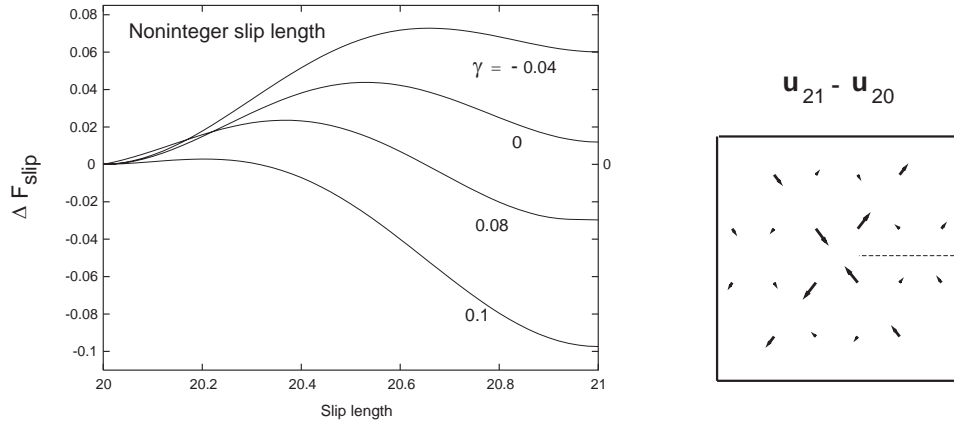
FIG. 3. Slip energy difference \Delta F_{\text{slip}}(\ell) in the range 20 \leq \ell \leq 21 for \gamma = -0.04, 0, 0.08 , and 0.1 in the model without free volume (left). Displacement difference \mathbf{u}_{21} - \mathbf{u}_{20} at \gamma = 0 needed for growth by unit length (right).
