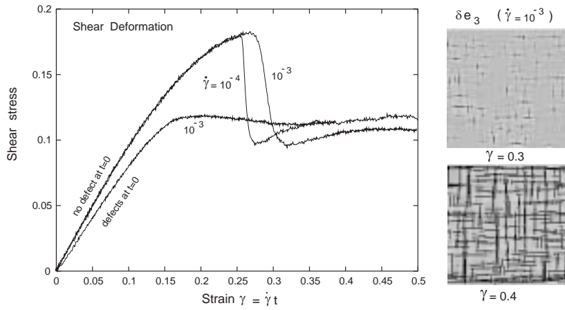
FIG. 1. Stress-strain curves from (2.6). Those at \dot{\gamma} = 10^{-4} and 10^{-3} without defects at t = 0 exhibit pronounced overshoot. Snapshots of \delta e_3 = e_3 - \gamma are given at \gamma = 0.3 and 0.4 (right). No marked overshoot appears in the other curve at \dot{\gamma} = 10^{-3} , where high-density dislocations are initially present.
