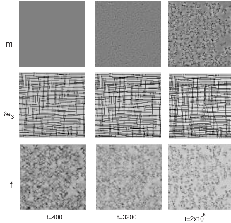
FIG. 7. Snapshots of free volume m , shear strain deviation \delta e_3 , and free energy density f at t = 400, 3200 , and 2 \times 10^5 for \langle m \rangle = 0.2 , showing growth of heterogeneity of m , an increase of plastic strain, and a decrease of f .
