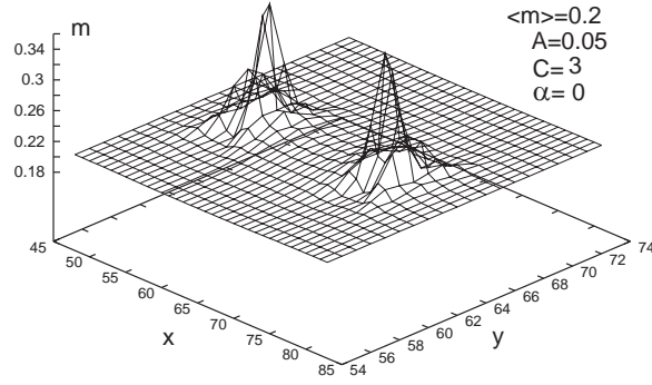
FIG. 5. Free volume m accumulated at the dislocation cores due to m -dependence of the shear modulus.
