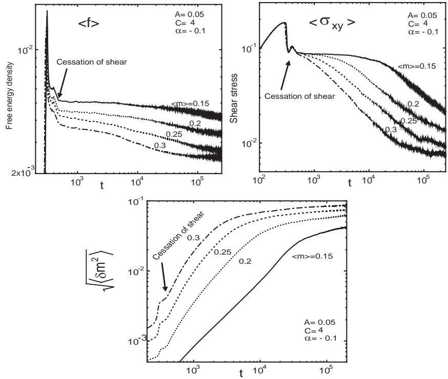
FIG. 6. Free energy density \langle f \rangle(t) , shear stress \langle \sigma_{xy} \rangle(t) , and free-volume variance \sqrt{\langle \delta m^2 \rangle}(t) vs t . A shear flow with \dot{\gamma} = 10^{-3} is applied in the time region 0 < t < 400 and is stopped at t = 400 . Relaxations become apparent with increasing the average free volume \langle m \rangle .
