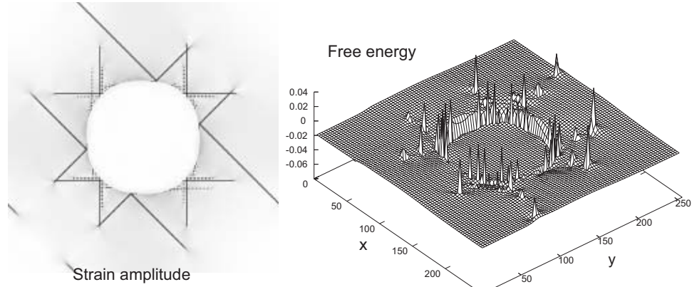
FIG. 9. Strain amplitude \epsilon (left) and free energy density f (right) around an incoherent hard domain. Here \epsilon is zero within the hard domain and nonvanishing outside. The peaks of f are located at the dislocation cores.
