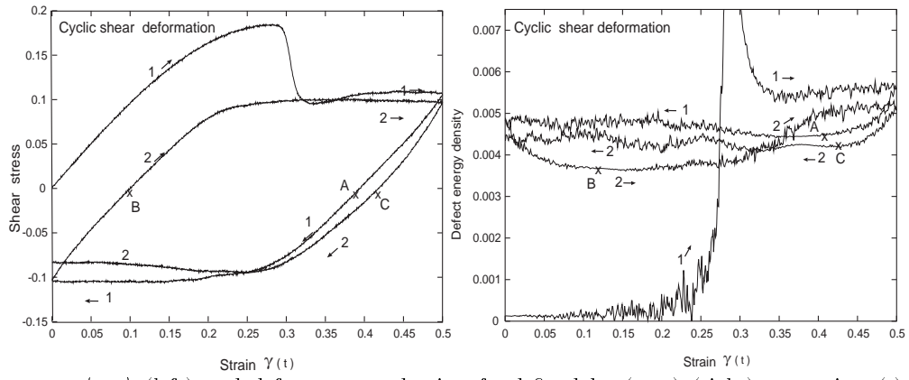
FIG. 4. Shear stress \langle \sigma_{xy} \rangle (left) and defect energy density f_D defined by (2.12) (right) vs strain \gamma(t) for cyclic shear deformation at \dot{\gamma} = \pm 10^{-3} . The shear stress vanishes at the three points A, B, and C ( \times ).
