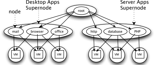
Figure 2: Tree model example
