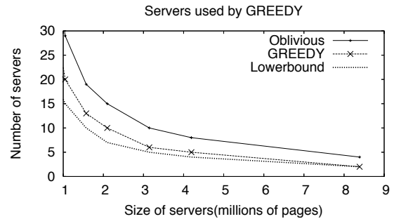
Figure 4: Comparison of server usage
